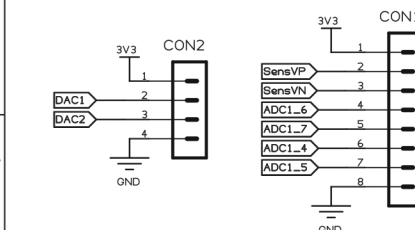
DAC ADC connector
