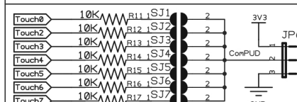
Pull Up/Down resistors
