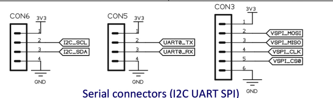
Serial connectors (I2C UART SPI)
