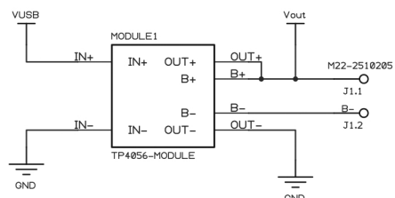
LiPo charger
