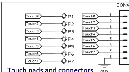
Touch pads and connectors
