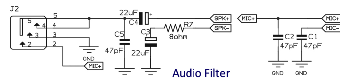
Audio Filter
