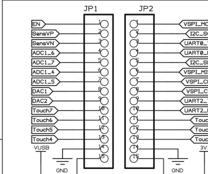
Connectors Breakout
