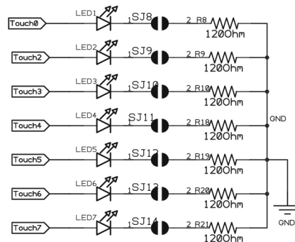
LED indicators
