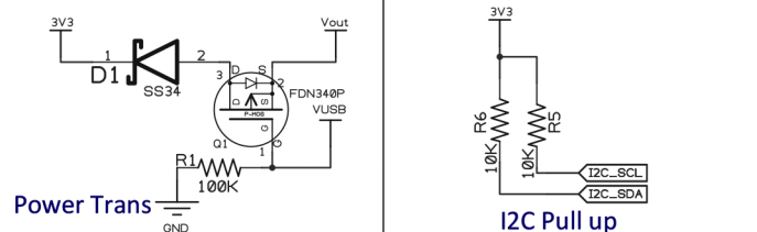
I2C Pull up
